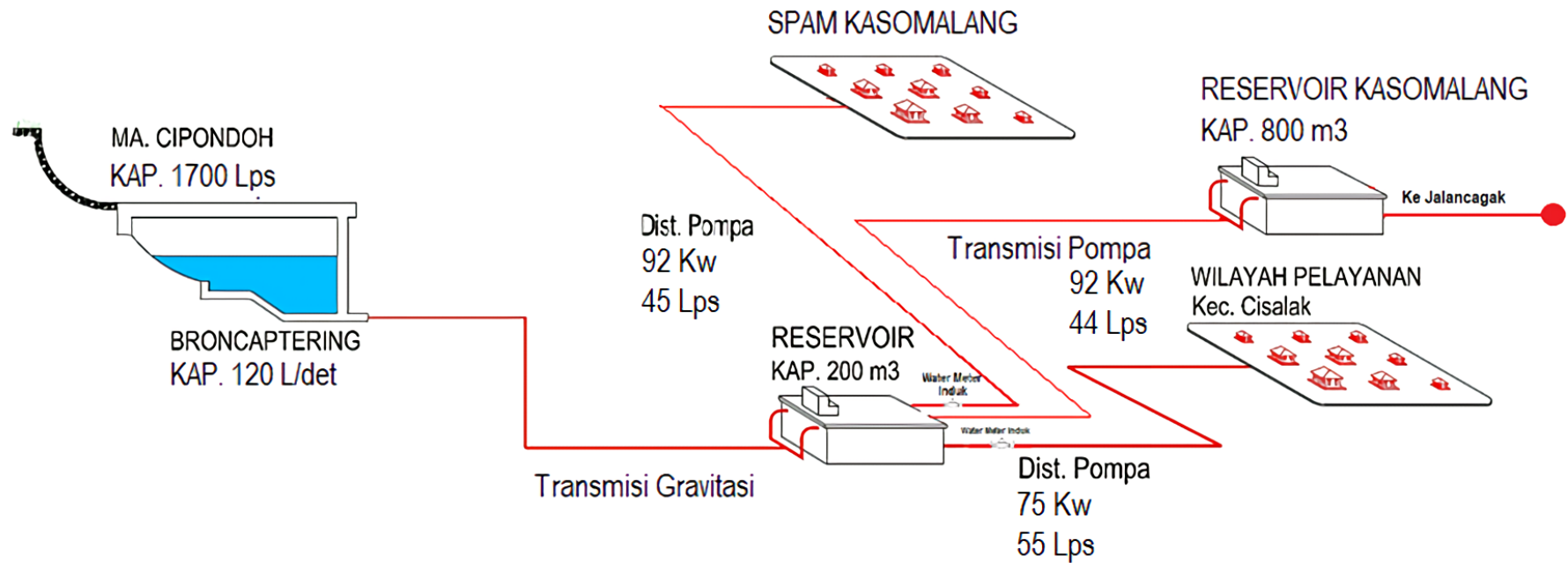
SKEMATIK SPAM CISALAK
